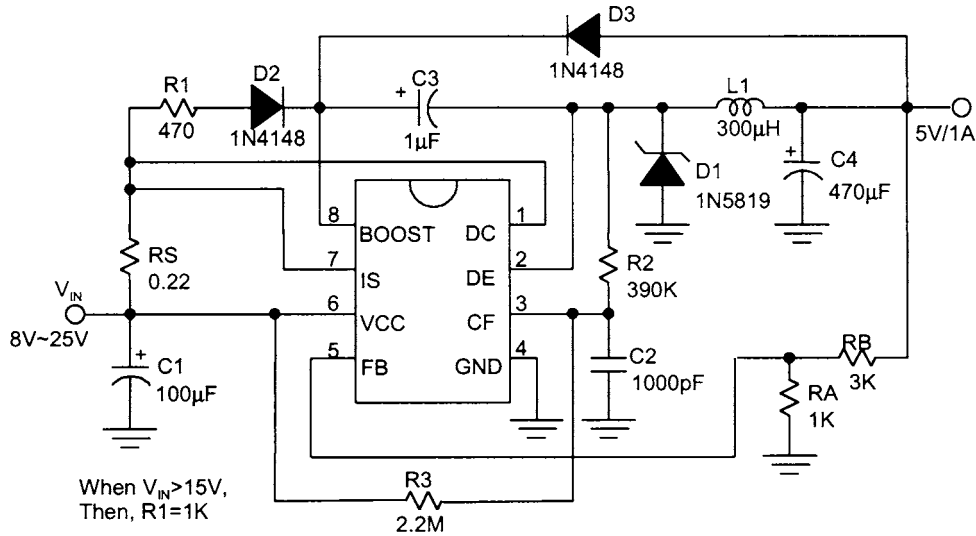
Fig. 3 Step-Down Converter
